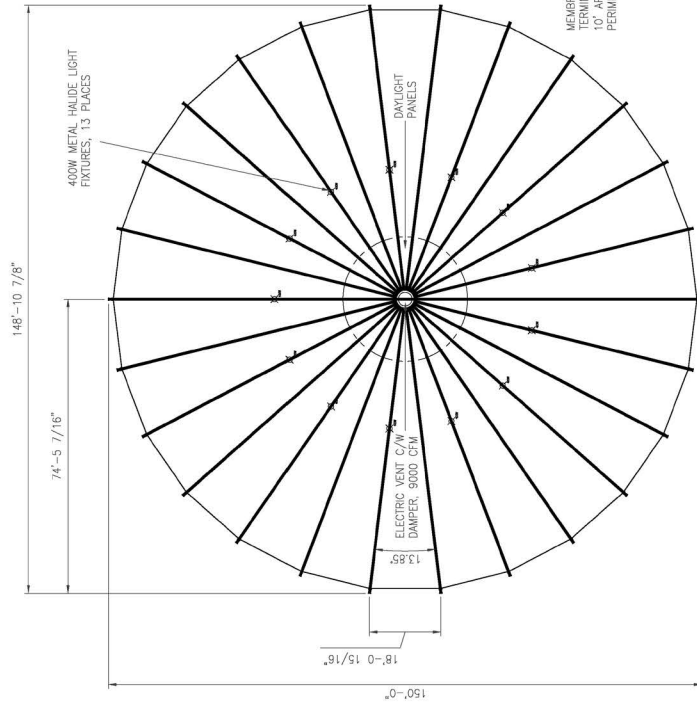
1 PLAN VIEW 201.0 1/16"=1'-0"
